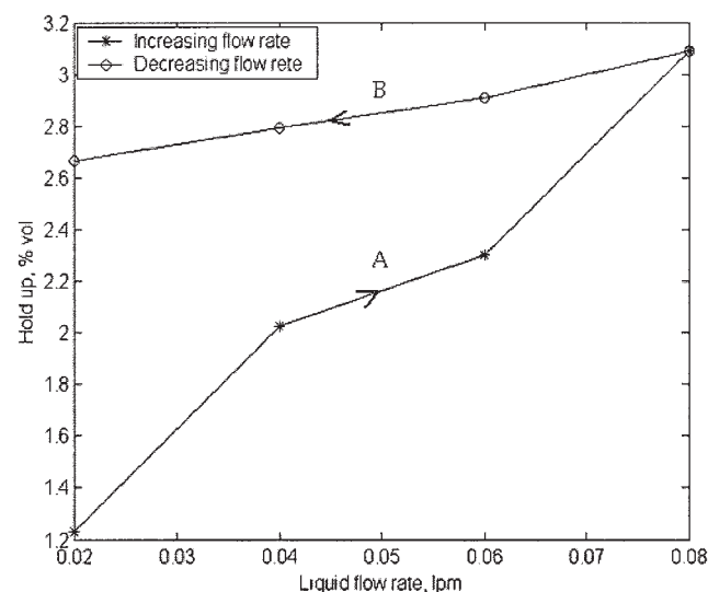
Figure 10. Experimental liquid hysteresis.
